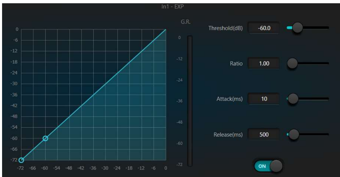
Fig.3.2 Expander
